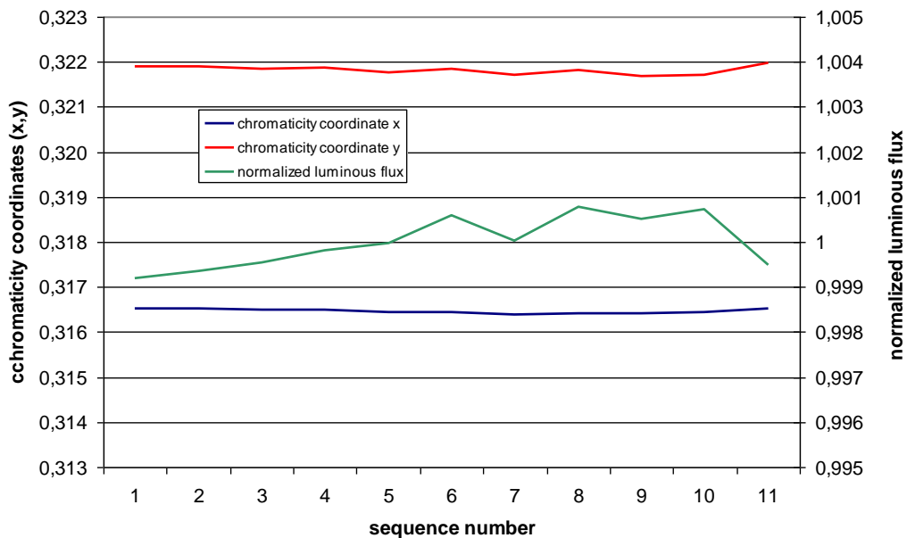
Fig. 3: Luminous flux (normalized) and chromaticity coordinates x,y for a group of 11 pulse trains
