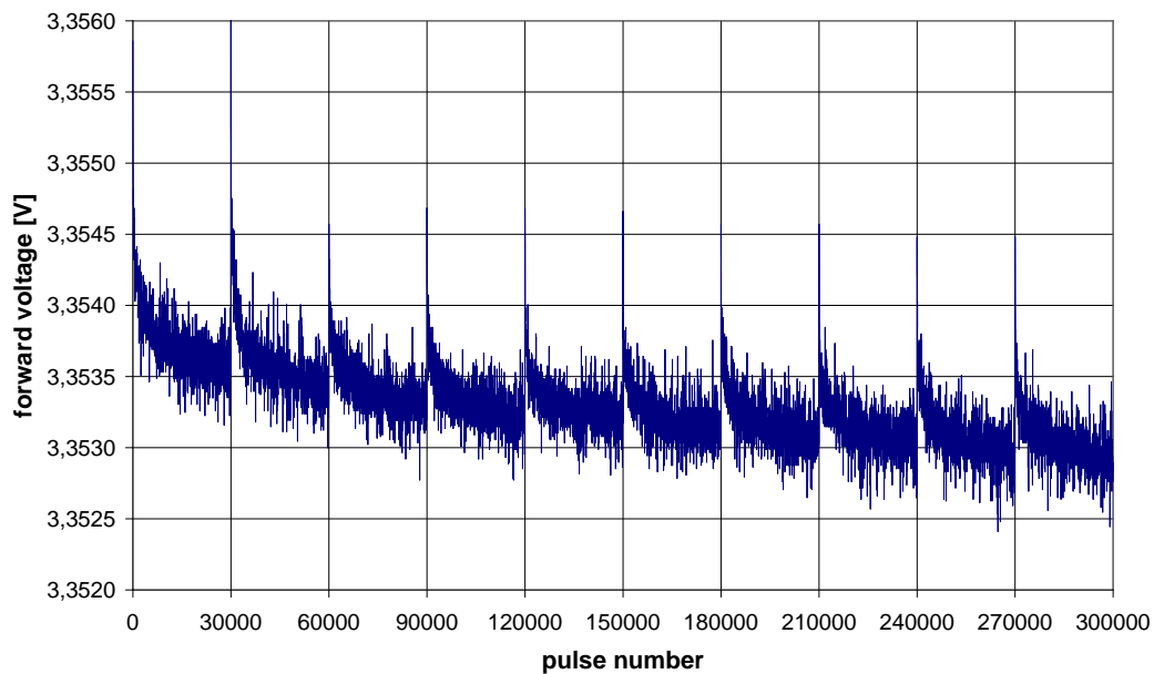
Fig. 2: Forward voltage of a white high-power LED, measured in pulsed mode
