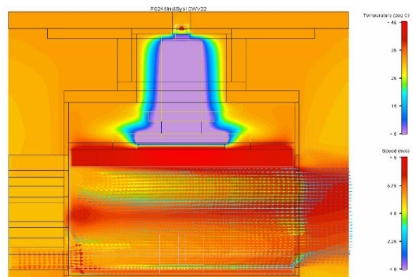
Fig. 1: Test fixture with Peltier based active cooling, FEM simulation of the heat sink
